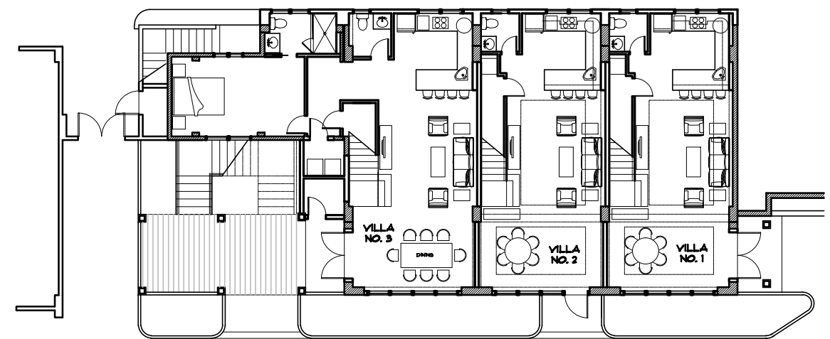
SECOND FLOOR PLAN SCALE: 1/8"=1'-0"
