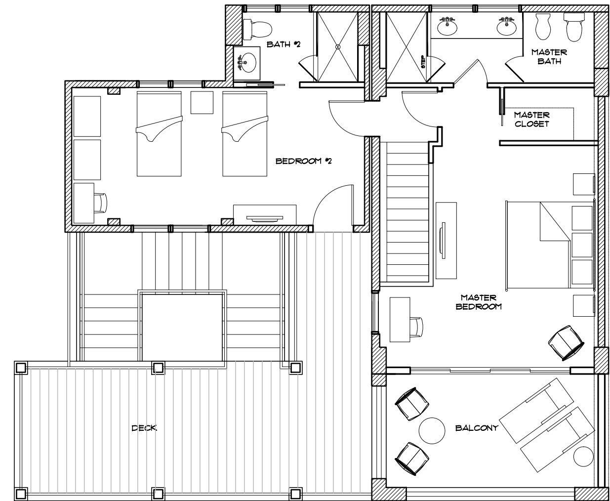
SECOND FLOOR PLAN SCALE: 1/8"=1'-0"
